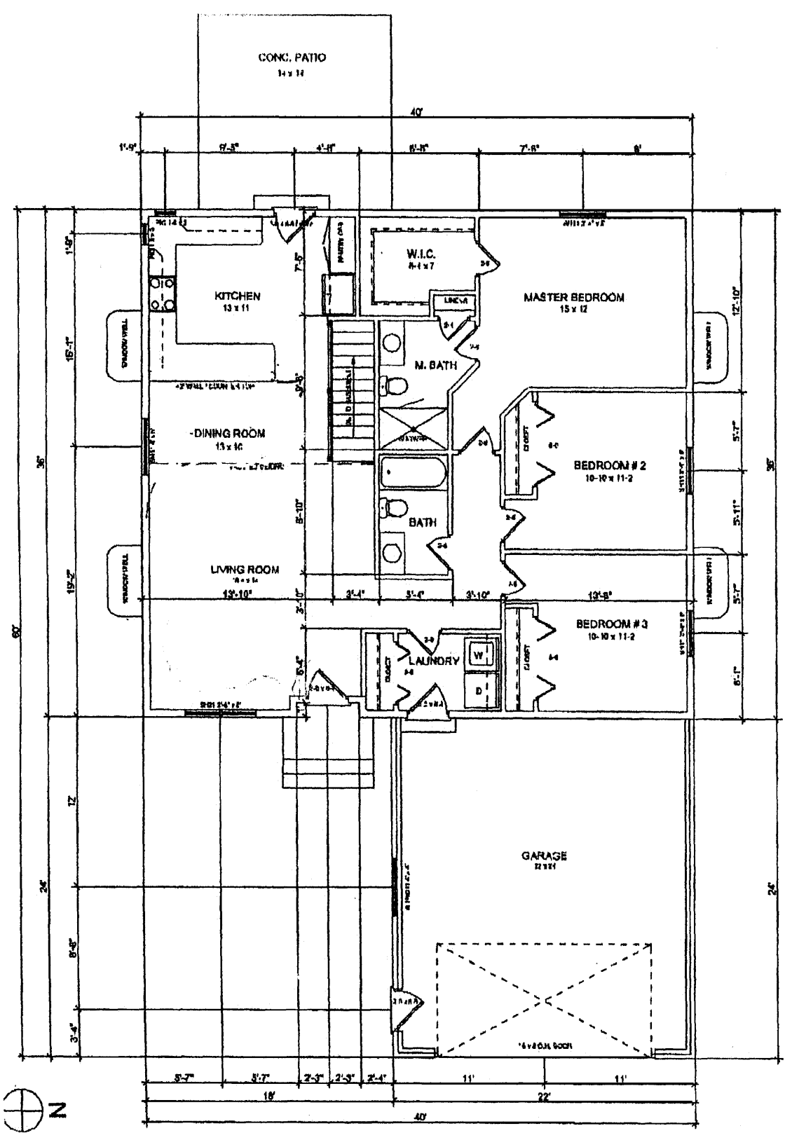
MAIN FLOOR PLAN = 1,440 SF. SCALE 1/4" = 1'-0"
